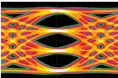
PAM4 Eye TX
